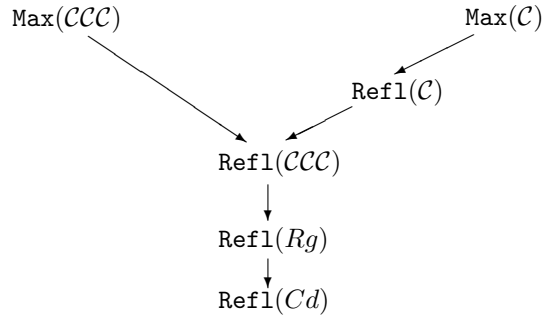
FIGURE 2. Reflection and maximality principles.
