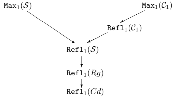
FIGURE 3. Reflection principles for 2^{\omega_1} .
